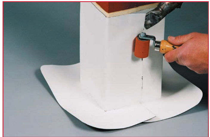
VersiWeld TPO Square Tubing Wraps are made of 45-mil reinforced VersiWeld membrane. A split (cut) and overlap tabs allow the seals to be opened and wrapped around square tubing.
