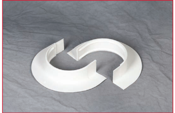
VersiWeld's Molded TPO Sealant Pockets consist of an interlocking, two-piece, injection molded flexible pocket with a rigid polypropylene vertical wall and preformed deck flanges. Used with Versico sealant and primer, this product effectively waterproofs pipe clusters or other odd shaped penetrations on VersiWeld roofing systems.
